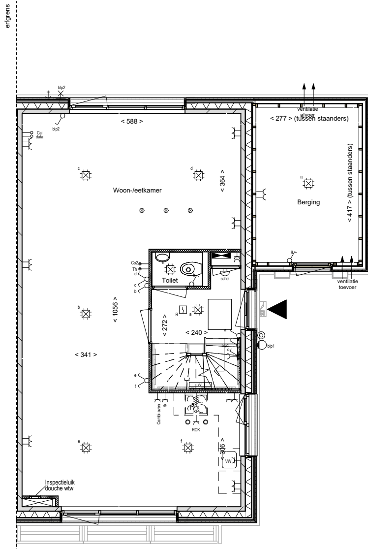
00 begane grond
